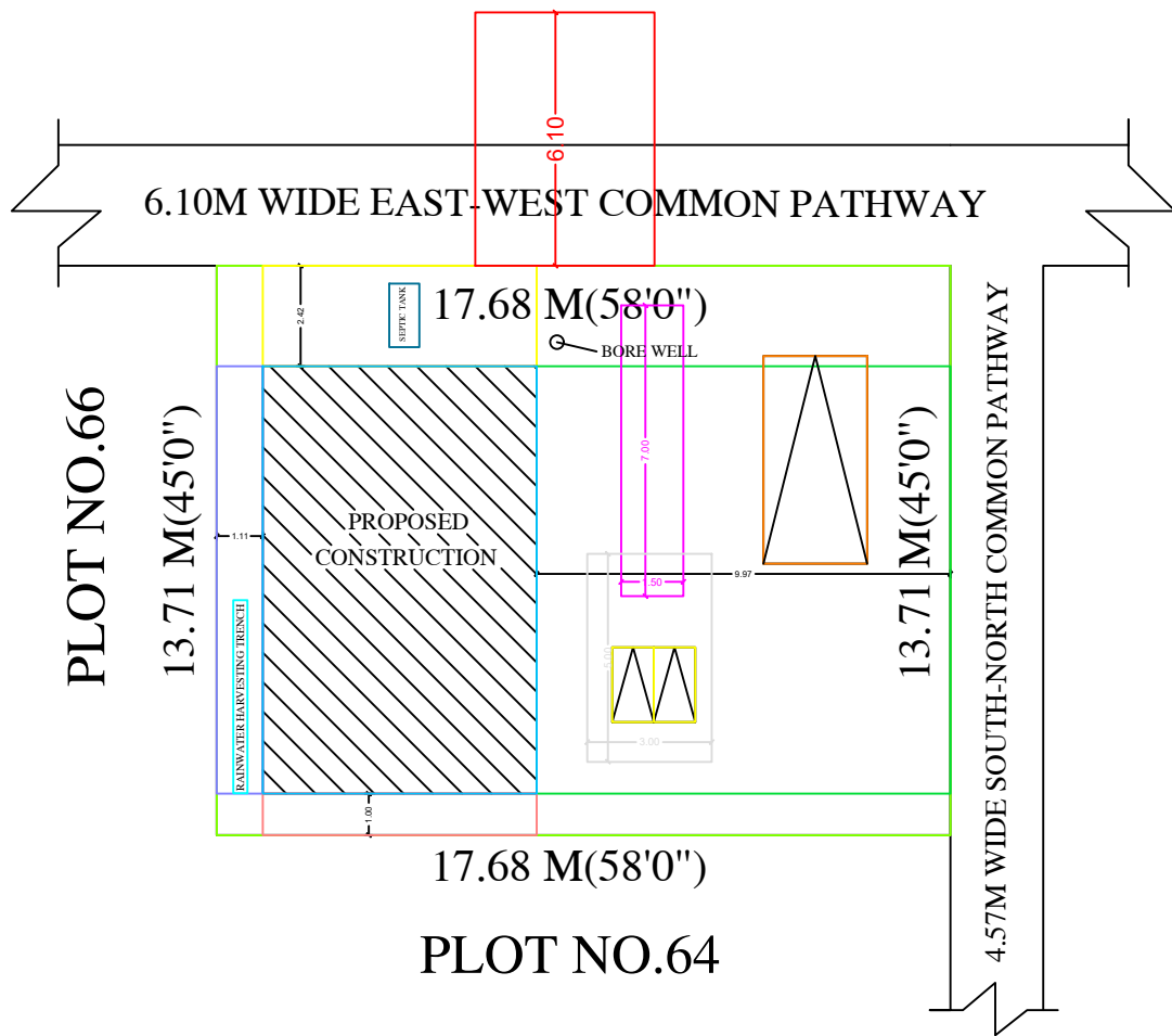
SITE PLAN
