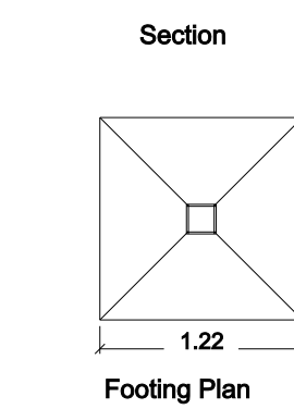
Footing Plan
