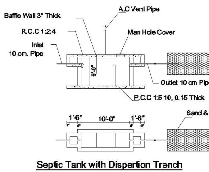
Sapic Tank with Dispersion Trench
