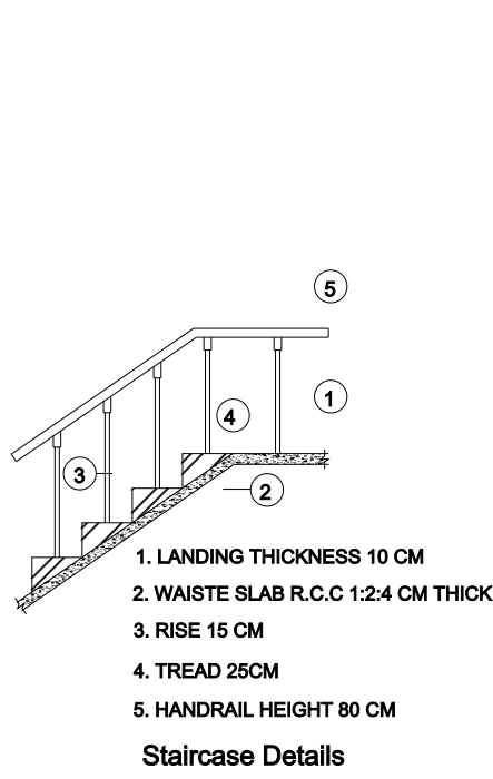
Staircase Details
