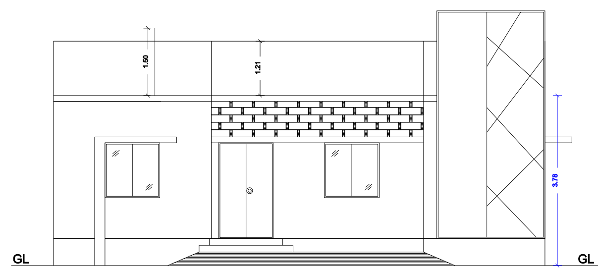
FRONT ELEVATION
