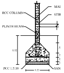
COLUMN DETAIL
