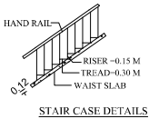
STAIR CASE DETAILS
