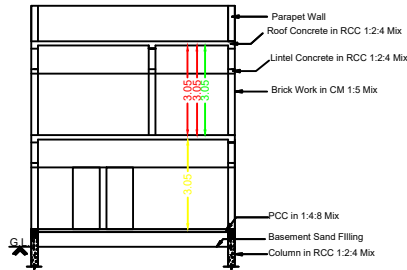
Section RR
