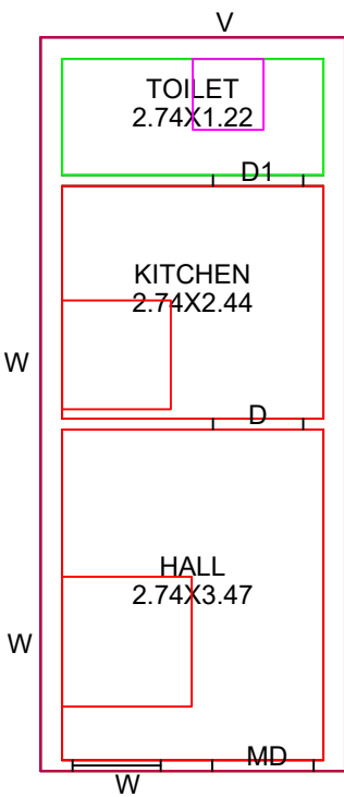
PRO.GROUND FLOOR PLAN
