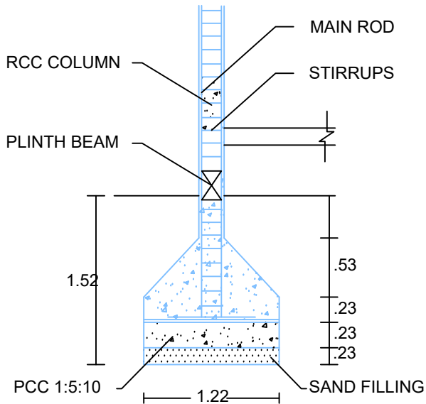
COLUMN DETAILS
