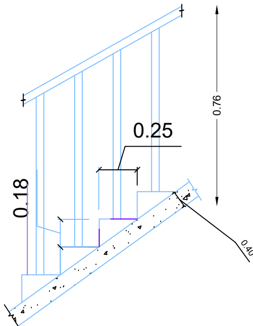
SECTION OF STAIRCASE
