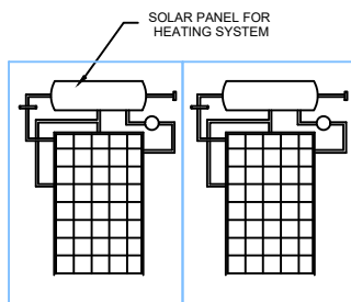
SOLAR HEATING SYSSEYM
