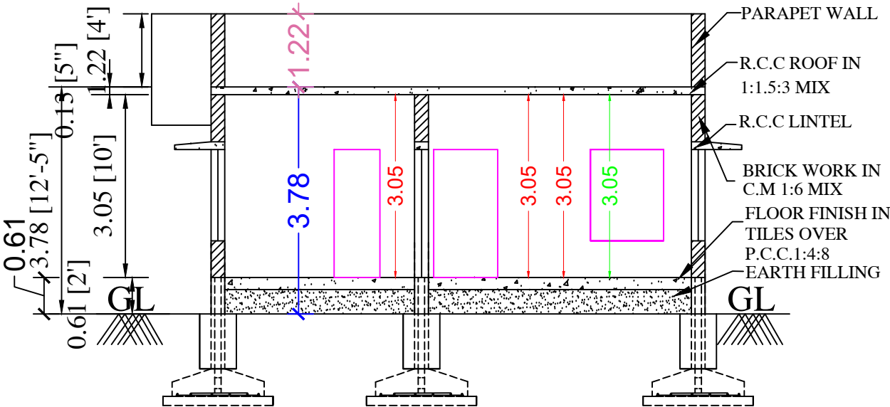
SECTION AA
