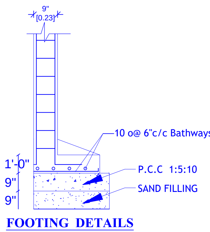
FOOTING DETAILS
