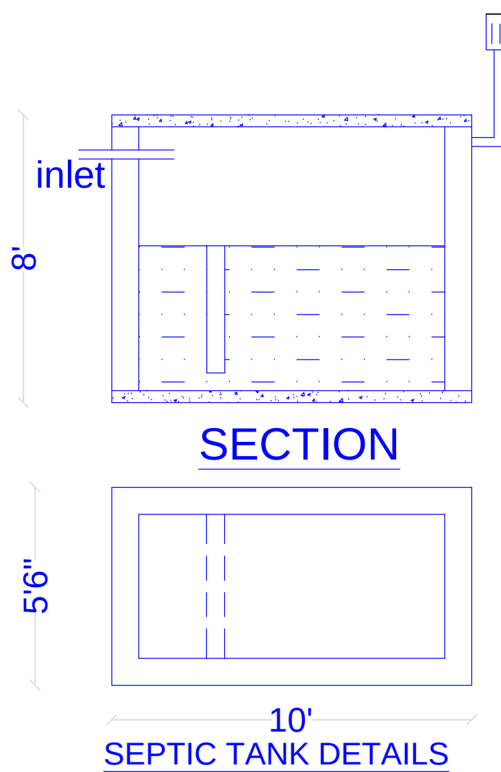
SEPTIC TANK DETAILS
