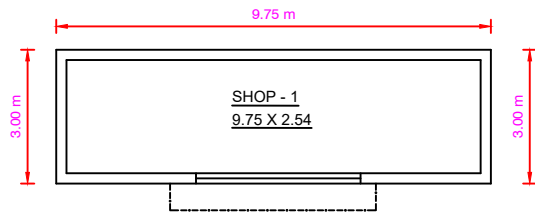
PROPOSED GROUND FLOOR PLAN
