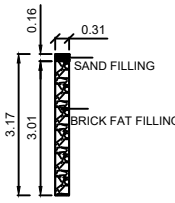
DETAILS OF PECULATION PIT
