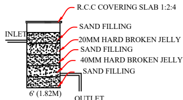
RAIN WATER HARVESTING SYSTEM
