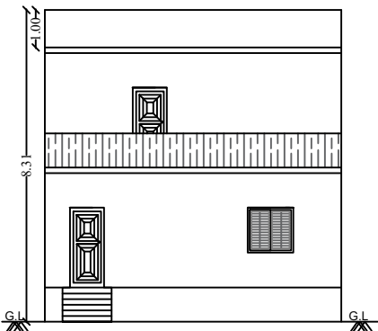
FRONT ELEVATION
