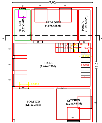
PROPOSED GROUND FLOOR
