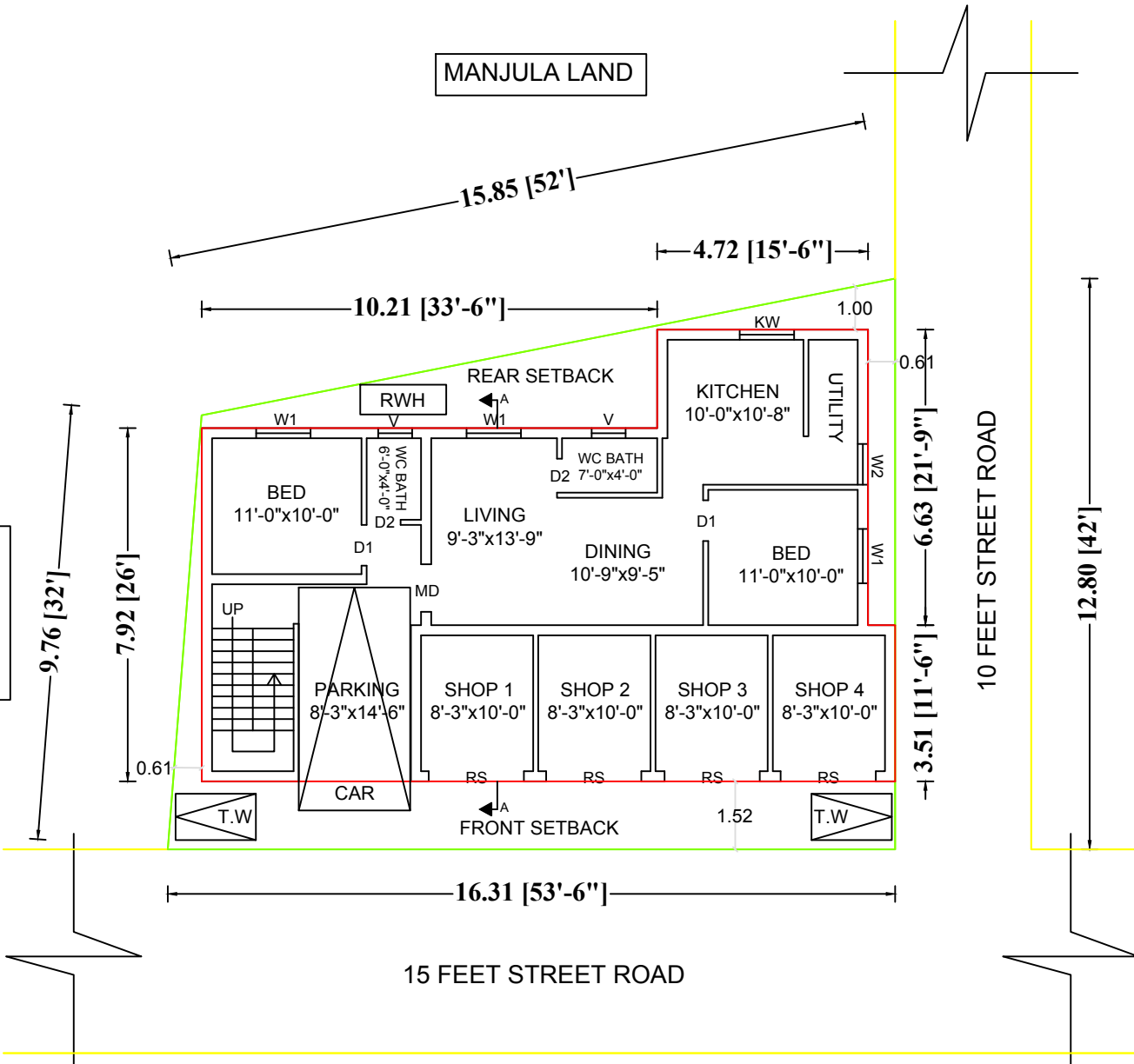
SITE CUM GROUND FLOOR PLAN (SCALE-1:100)
