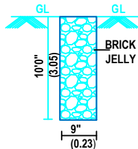
PERCULATION PIT
