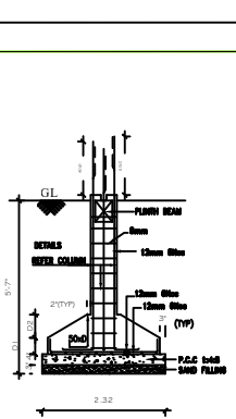
FOUNDATION DETAILS SCALE : 1:50.
