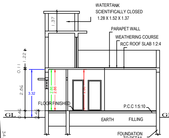
SECTION "A-B"
