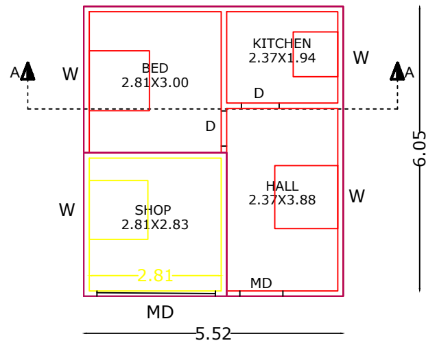
PROPOSED COMMERCIAL GROUND FLOOR PLAN & PROPOSED RESIDENTIAL GROUND FLOOR PLAN
