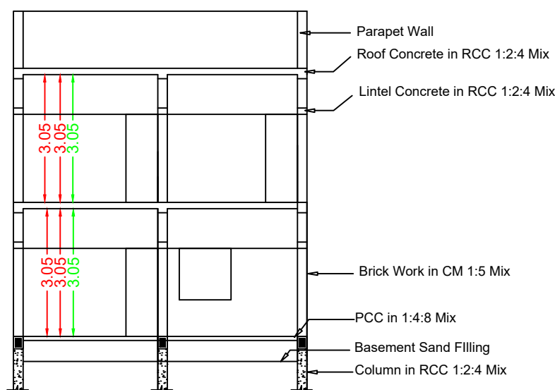
Section RR
