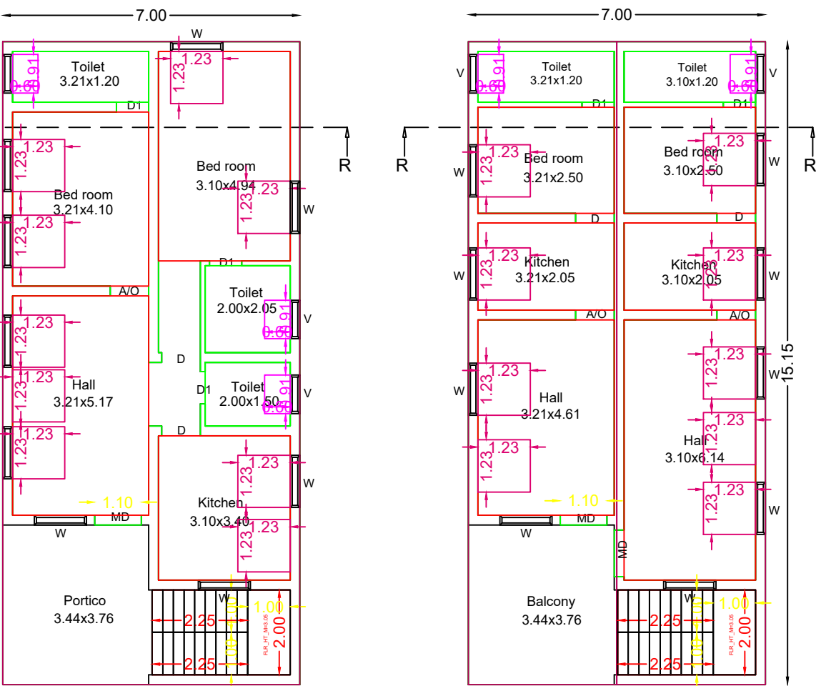
Pro.Ground & First Floor Plan
