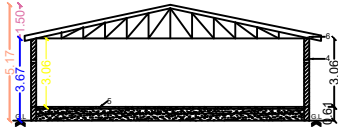
SECTION ON "AA"
