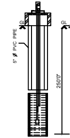
BOREWELL DETAILS
