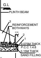
UMN FOOTING
