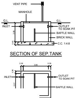
TANK
