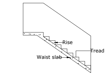
DETAIL OF STAIRCASE
