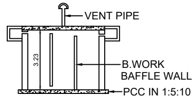
SECTION
