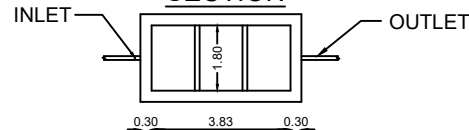
SEPTIC TANK DETAILS
