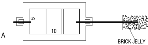
SEPTIC TANK & DISPERSION TRENCH DETAILS SCALE- 1:100
