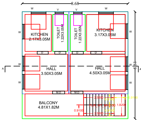
PROPOSED FIRST FLOOR
