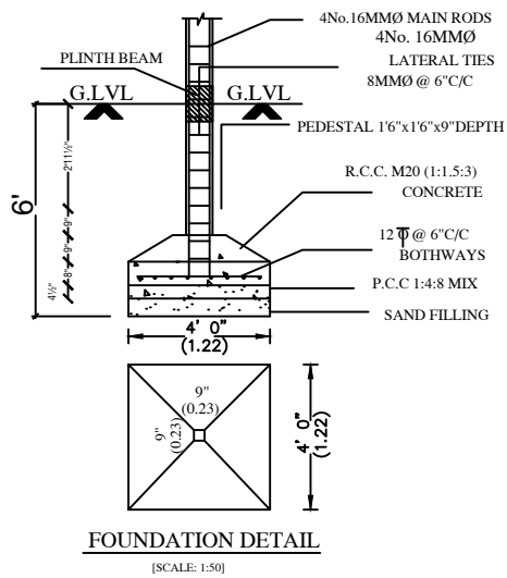
FOUNDATION DETAIL
