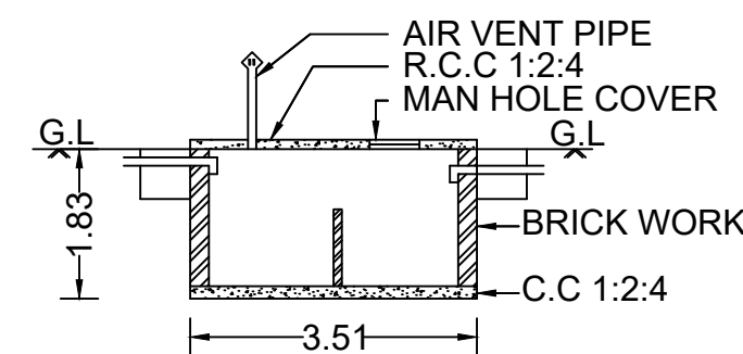
SEPTICTANK DETAILS
