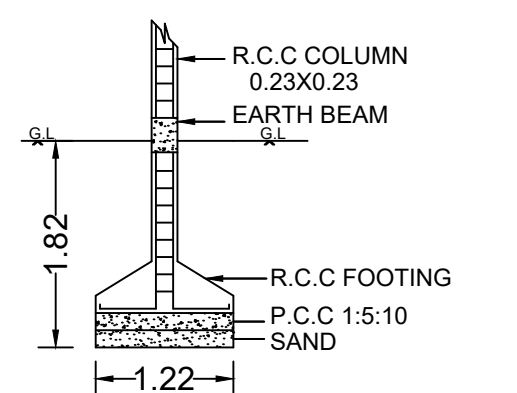
FOUNDATION DETAILS
