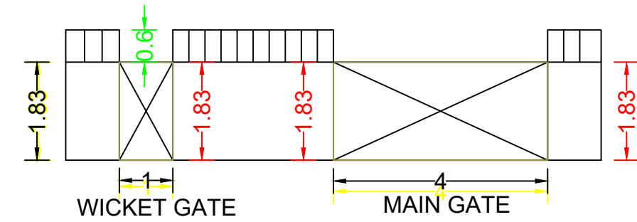
COMPOUND WALL
