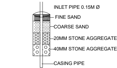
DETAILS OF RAIN WATER HARVESTING STRUCTURES
