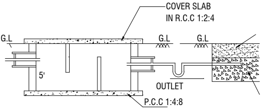
SECTION-AB
