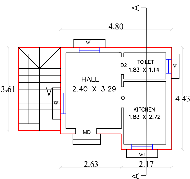
EXISTING AND PROPOSED GROUND FLOOR PLAN
