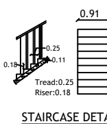
STAIRCASE DETAIL
