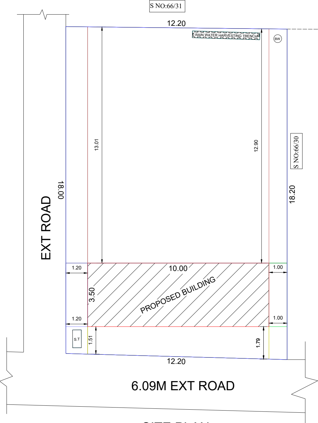
SITE PLAN
