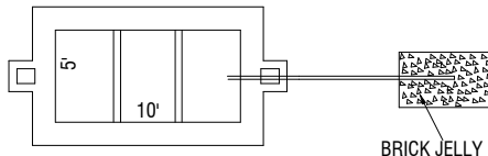
SEPTIC TANK & DISPERSION TRENCH DETAILS
