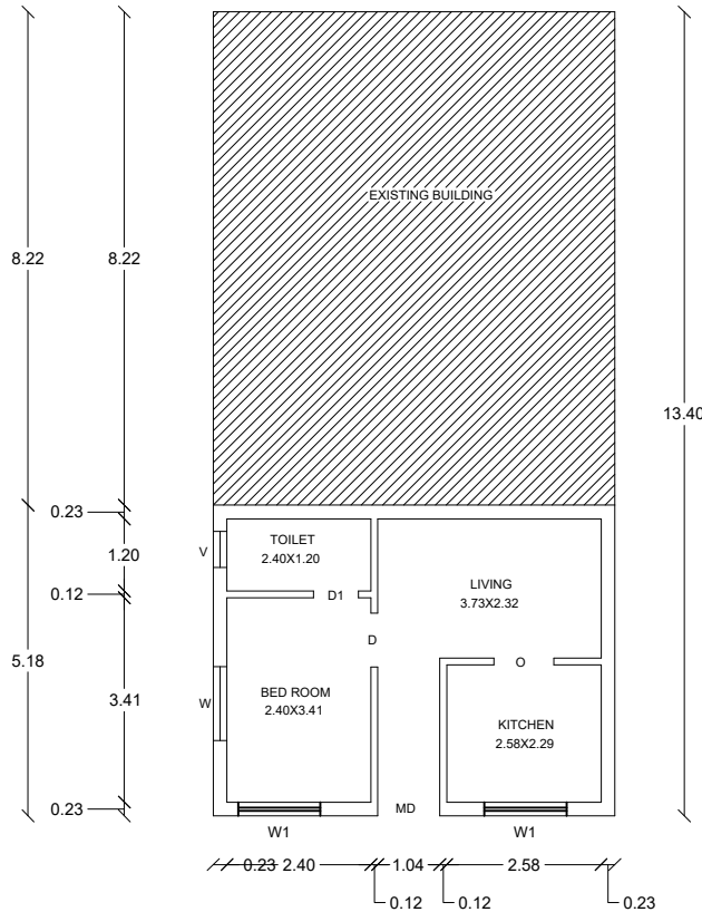
EXT & PRO GROUND FLOOR
