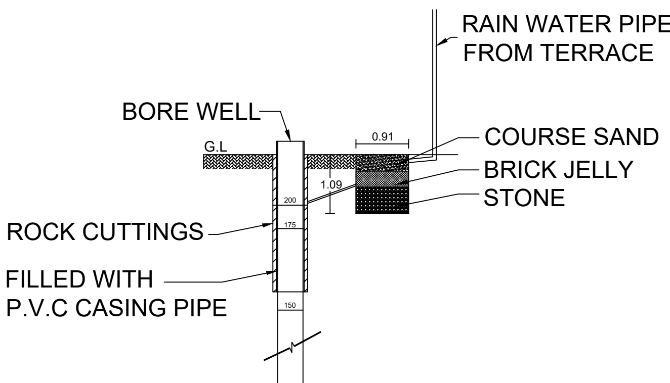
RAIN WATER HARVESTING DETAIL
