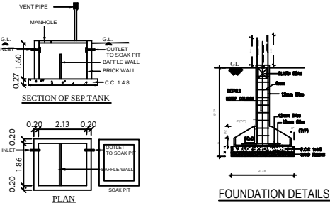
SEPTIC TANK
