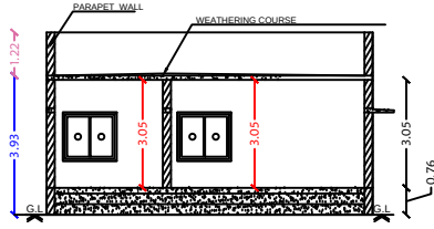
Section on-AA
