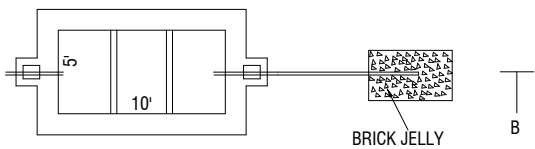
SEPTIC TANK & DISPERSION TRENCH DETAILS
