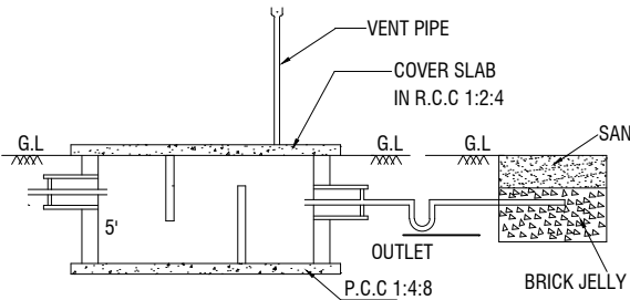
SEPTIC TANK & DISPERSION TRENCH DETAILS
