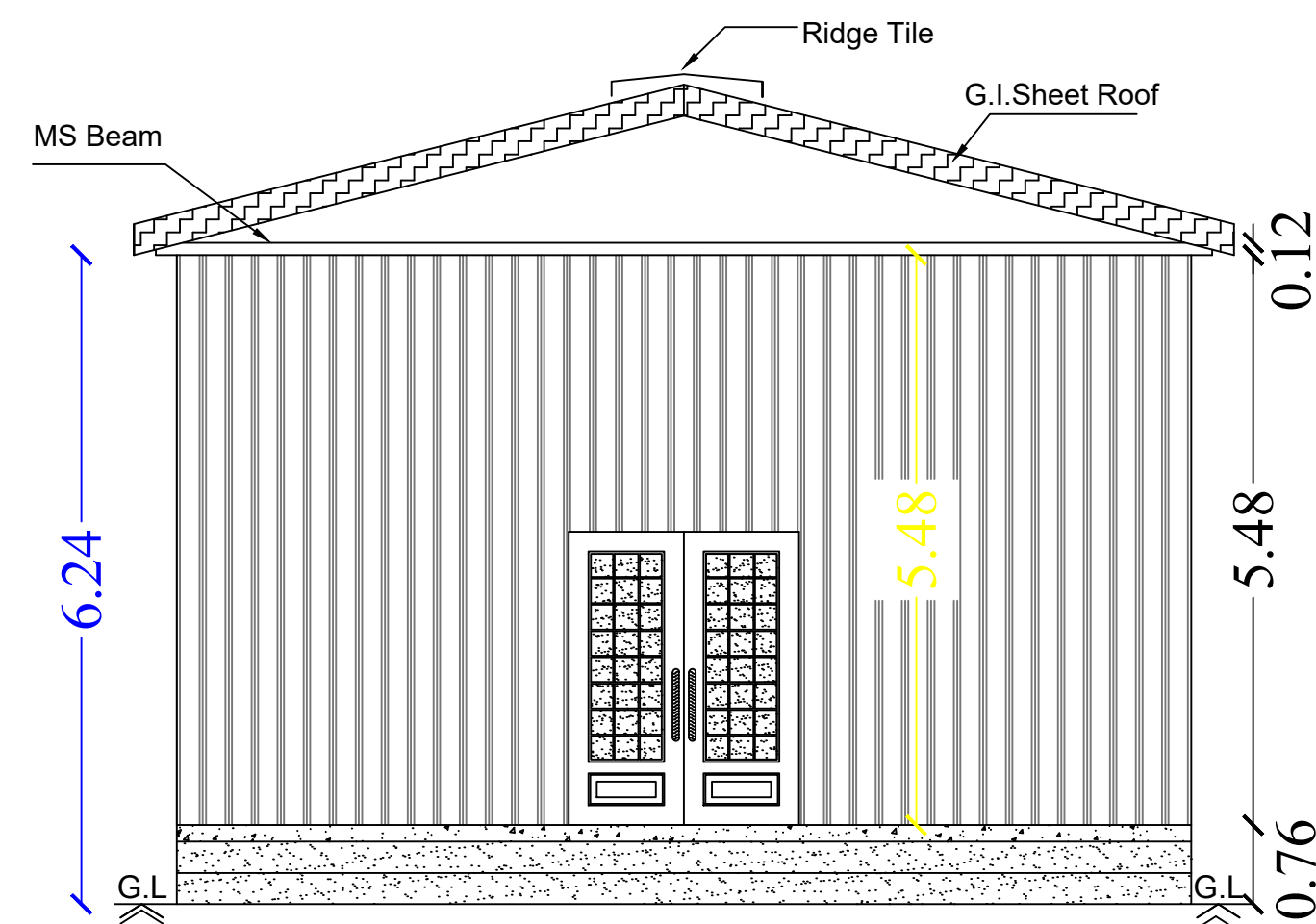
Section on-"AA"
