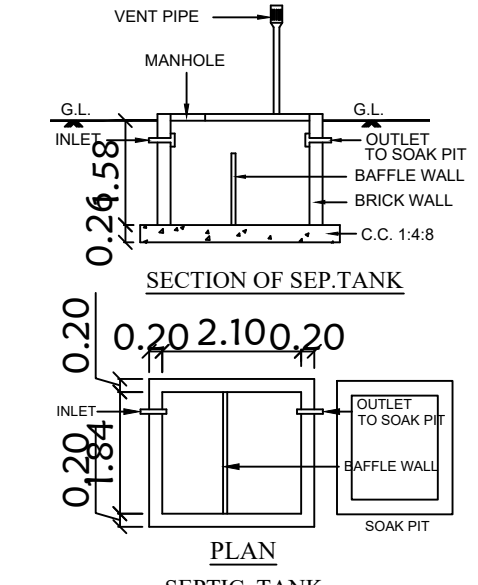
SEPTIC TANK
