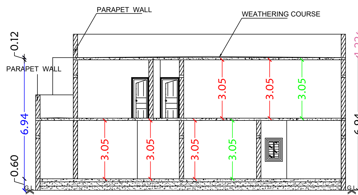
Section on-"AA"
