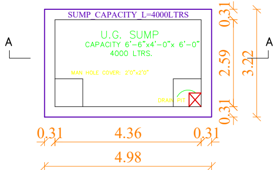
SUMP_DETAIL
