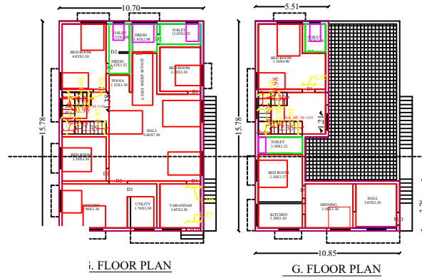
F. FLOOR PLAN
