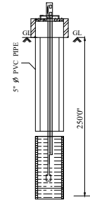
BOREWELL DETAILS
