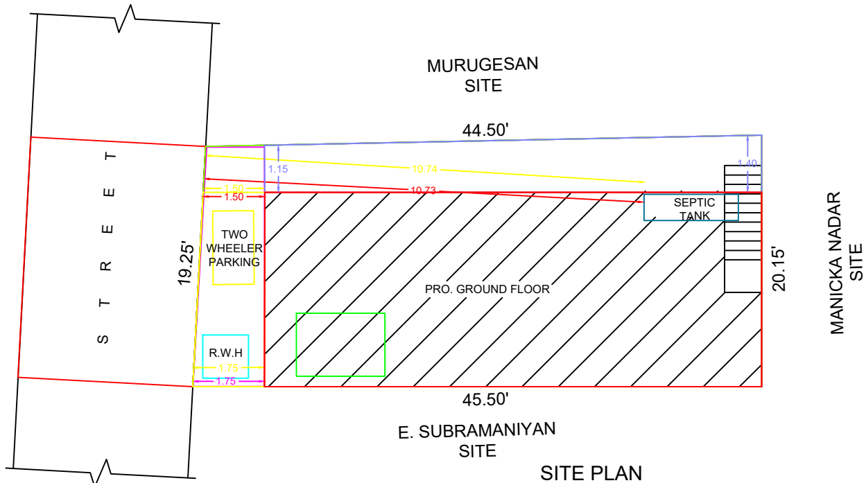
SITE PLAN
