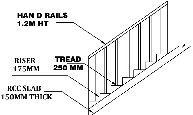
STAIRCASE DETAILS SCALE 1:50
