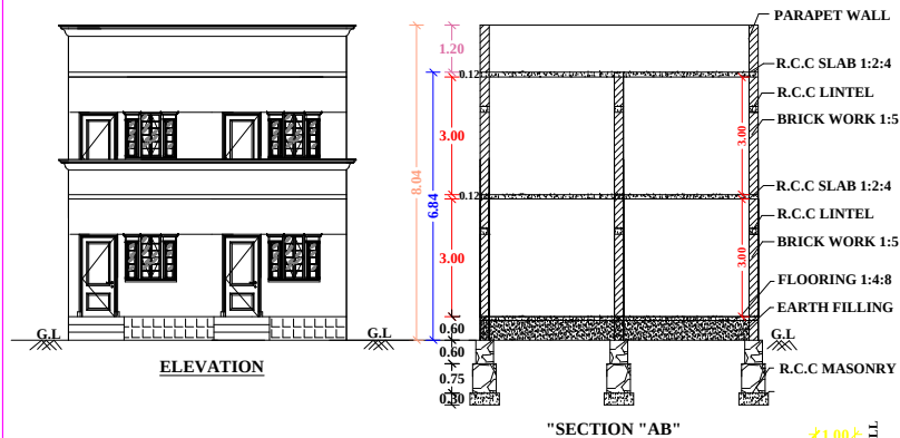
"SECTION AB"
