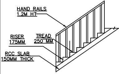
STAIRCASE DETAILS SCALE 1:50
