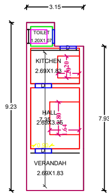
PLAN
