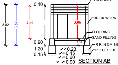
SECTION AB
