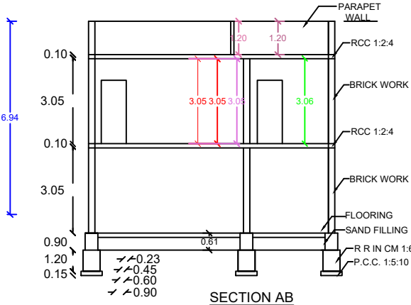
SECTION AB
