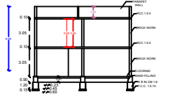
SECTION AB
