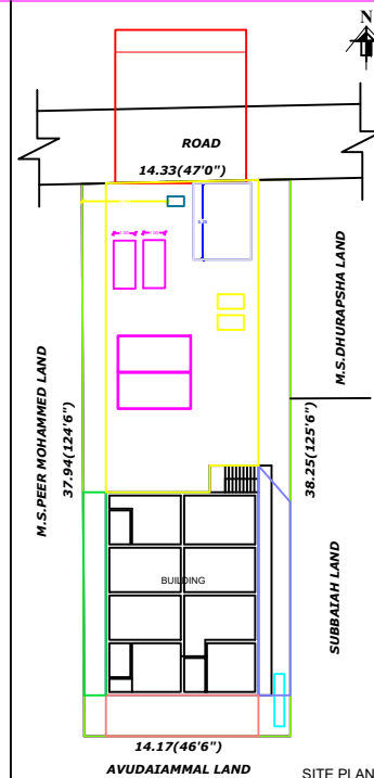
SITE PLAN
