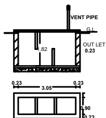
SEPTIC TANK
