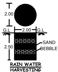
SECTION ON 'AB'
