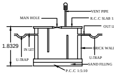
SECTION E.F. SEPTIC TANK DETAIL
