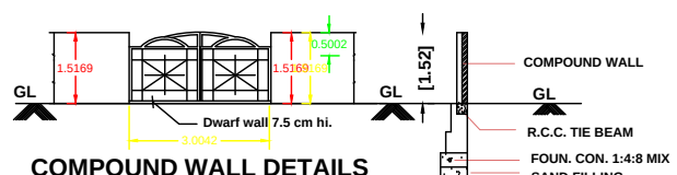
COMPOUND WALL DETAILS
