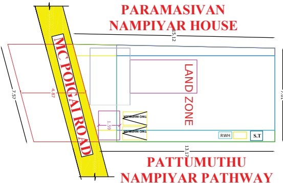
SITE PLAN
