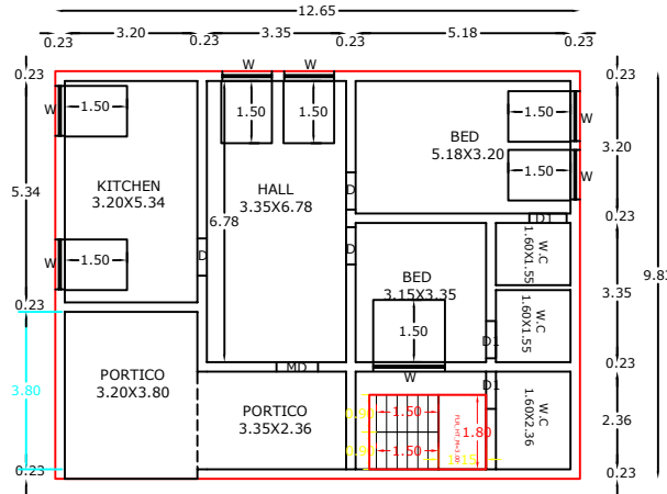
EXT GROUND FLOOR RESIDENTIAL PLAN
