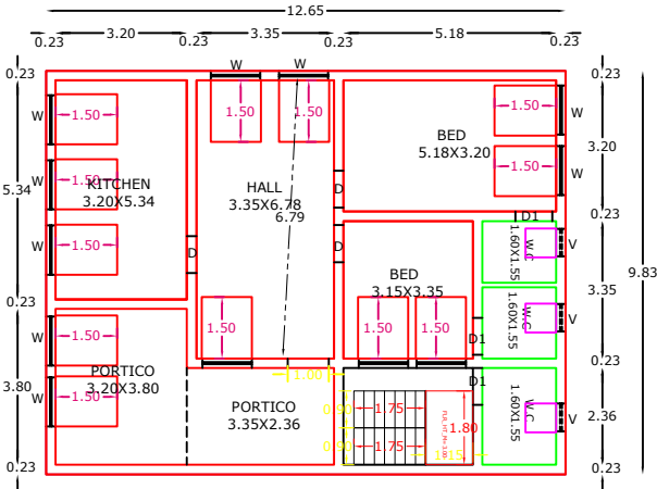
PRO FIRST FLOOR RESIDENTIAL PLAN
