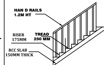
STAIRCASE DETAILS SCALE 1:50
