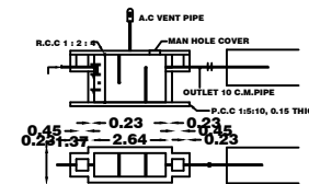
SEPTIC TANK & TRENCH
