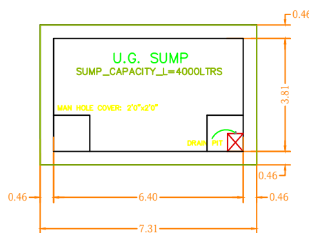
SUMP DETAIL SCALE 1"=4'-0"
