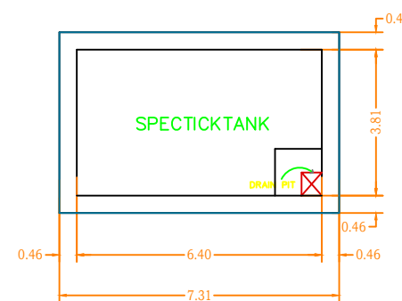
SPECTICK TANK DETAIL SCALE 1"=4'-0"
