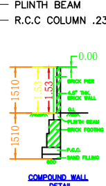
COMPOUND WALL DETAIL
