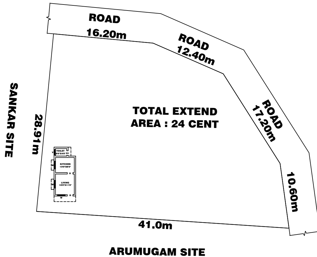
SITE PLAN SCALE 1:300
