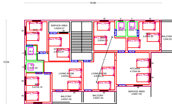
PRO. SEC. FLOOR PLAN
