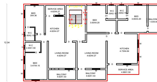
EXT. FIRST FLOOR PLAN
