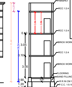
SECTION AB
