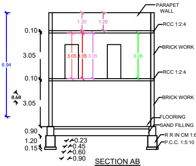
SECTION AB
