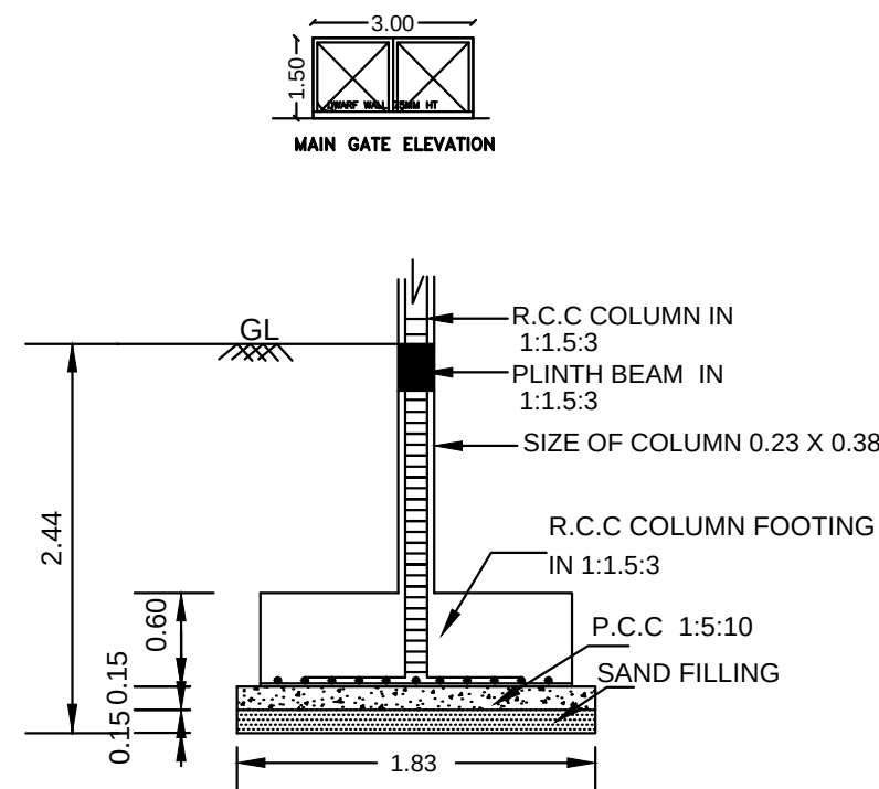
FOUNDATION DETAIL-A
