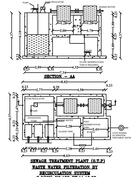
SEWAGE TREATMENT PLANT (S.T.P.)
