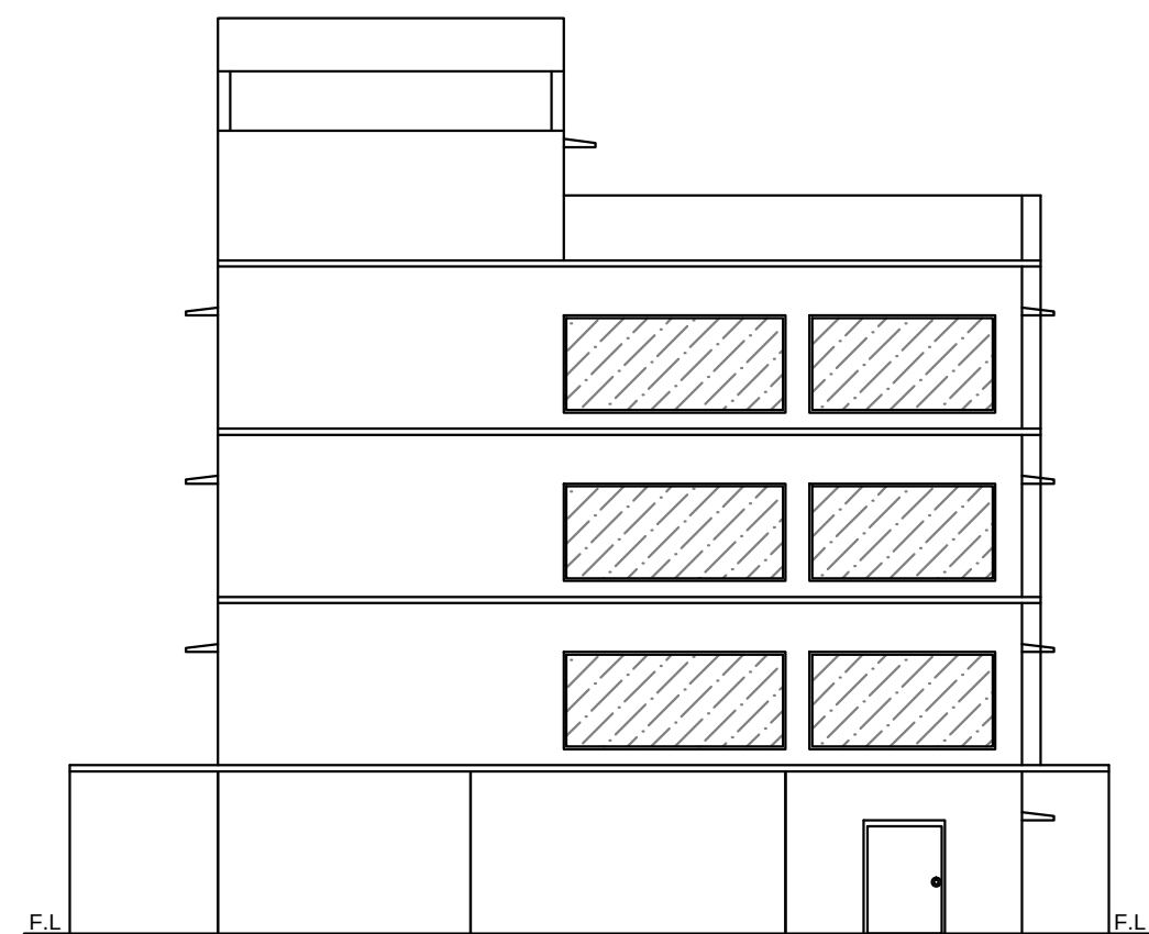
FRONT ELEVATION
