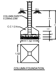
COLUMN FOUNDATION
